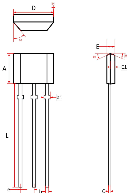
TO-92S
